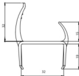
PVC PROFİL 32MM (SİYAH - BEYAZ , GRİ - BEYAZ) PVC PROFILE (BLACK - WHITE, GREY - WHITE)
