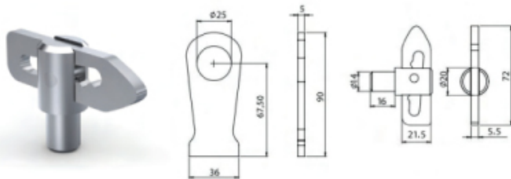
TIRTILLI KİLİT GALVANİZ / OPEN BOX LOCK
