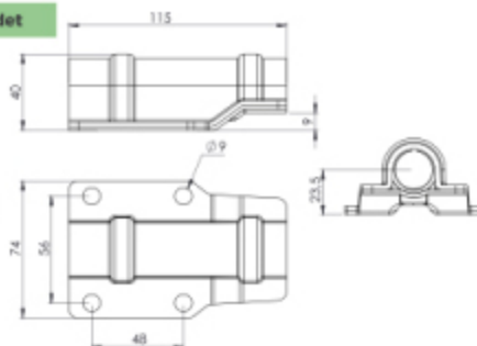
BÜYÜK BORU YUVASI GALVANİZ Ø22 / BIG GUIDE PLATE Ø22 (ZP)
