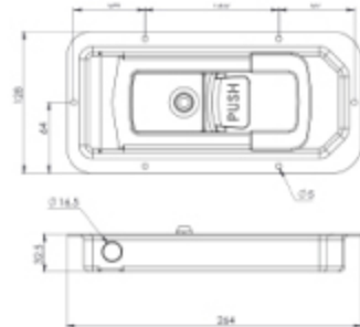
KÜÇÜK GÖMME KİLİT ASMA KİLİTLİ KROM - GALVANİZ SMALL RECESSED DOOR LOCK WITH PADLOCK (SS) - (ZP)
