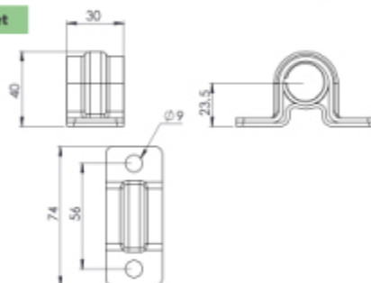
KÜÇÜK BORU YUVASI GALVANİZ Ø22 / SMALL GUIDE PLATE Ø22 (ZP)
